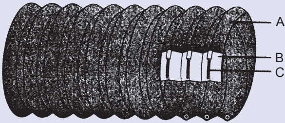
A Outer ply polyurethane. B Inner ply polyurethane. C PVC coated spring steel helix.
