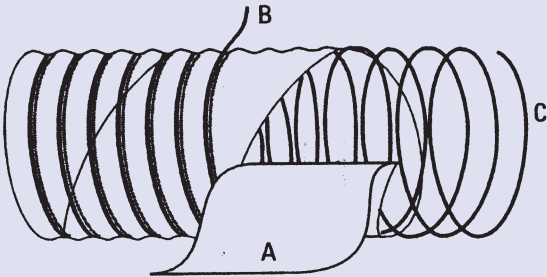
A Neoprene coated fibreglass. B Neoprene coated fibreglass cord. C spring steel helix.
